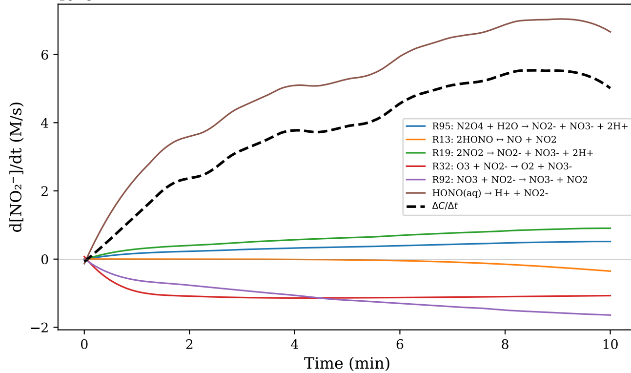
(c) \text{NO}_2^-
